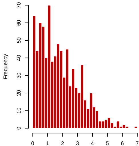
truncated: only y > 0 recorded
