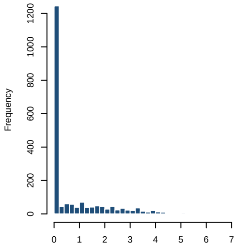
censored: y = \max(0, y^*)
